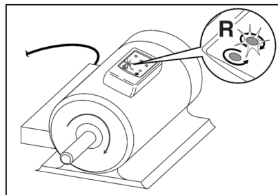
Figure 3. Motor Rotation
