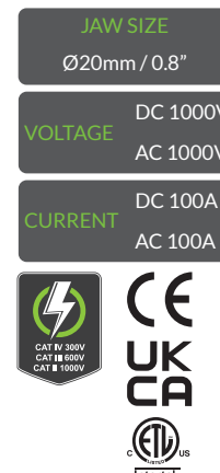
DCM400LEAK AC/DC TRMS leakage Clamp Meter
